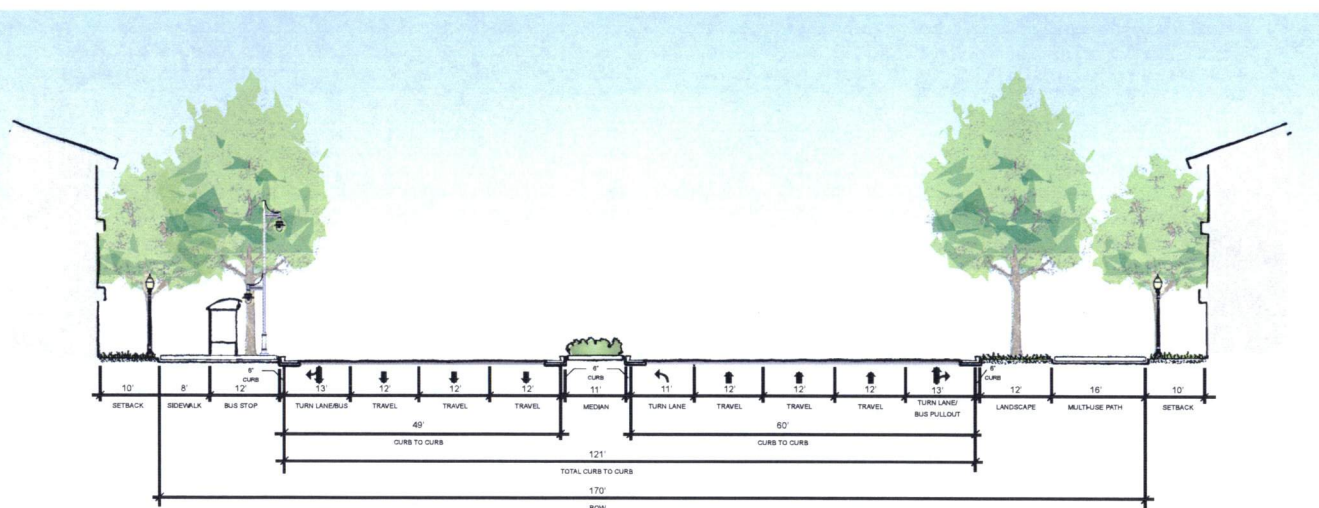
C US 29 Six Lane with Urban Frontage
