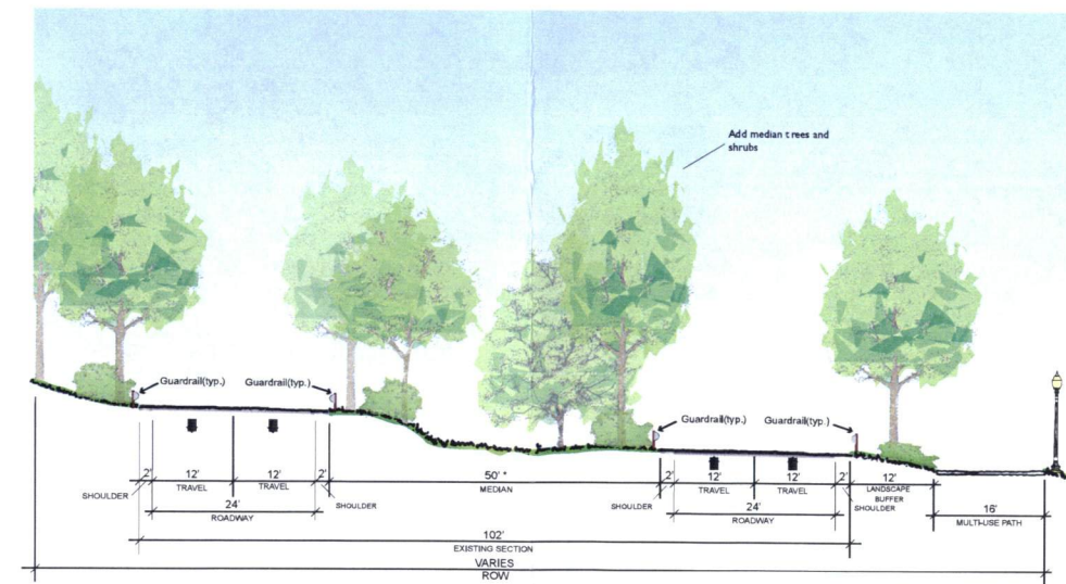
F US 29 Existing Conditions with added Multi-Use Path and Median Landscaping
