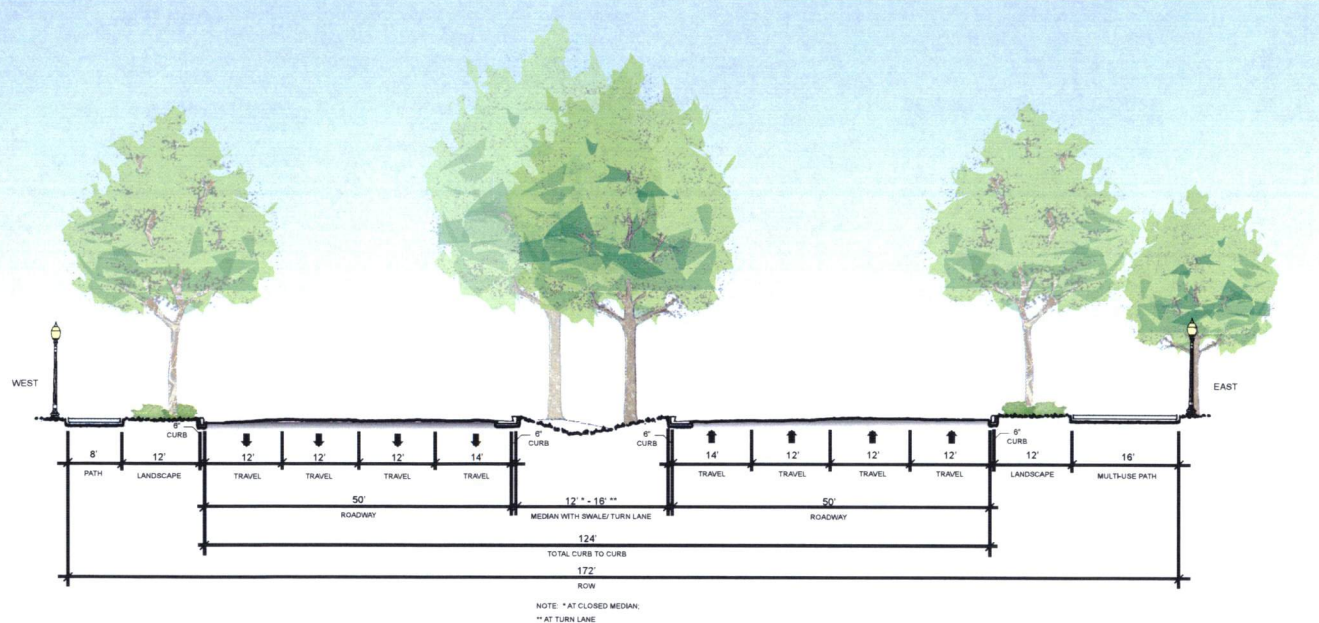
A US 29 Eight Lane Section (Typical)
